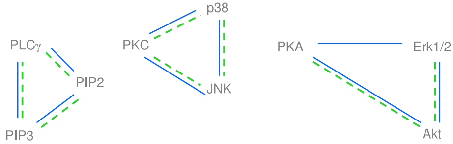
Fig. 3. Inferred graphs. The graphs estimated with the methods of Drton and Perlman and Wille and Bühlmann are identical and represented in blue. The graph estimated with the method of Meinshausen and Bühlmann is in green dotted line
